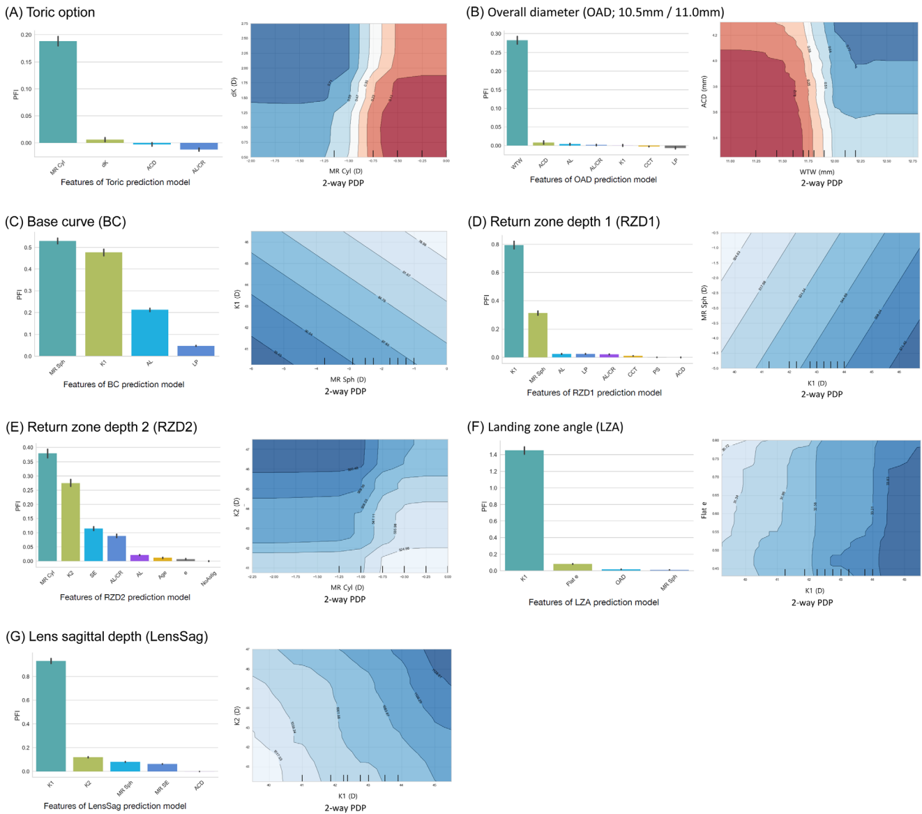
Figure 7. Permutation feature importance (PFI) estimates selected using the machine-learning method and two-way partial dependence plots (PDPs). (A) Toric option prediction based on cylindrical refraction (MR Cyl) and keratometry astigmatism (dK) values (threshold = 0.5; 0 = non-toric; 1 = toric). (B) OAD prediction based on WTW and ACD values (threshold = 0.5; 0 = 10.5 mm; 1 = 11 mm). (C) BC prediction based on MR Sph (spherical refraction) and K1 (flattest keratometry). (D) RZD1 prediction based on K1 (flattest keratometry) and MR Sph. (E) RZD2 prediction based on MR Cyl and K2 (steepest keratometry). (F) LZA prediction based on K1 and flat e (flat or horizontal eccentricity). (G) LensSag prediction based on K1 and K2.
