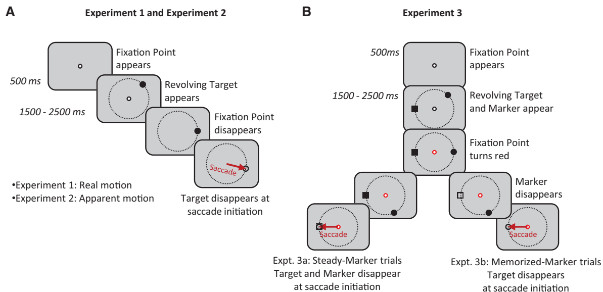
Figure 1. Schematic diagram of the experimental procedures. (A) Experiments 1 and 2. After 1500 to 2500 ms of central fixation, the fixation point disappeared, after which subjects made a saccade to a revolving target as quickly as possible. The target moved in real motion in Experiment 1 and apparent motion in Experiment 2. (B) Experiment 3. The procedure was similar to Experiments 1 and 2, but a stationary saccade target marker was also present on the target trajectory, and, after the fixation point turned red, a saccade was made to the location of the marker so that the eye would land on the marker at the time the target passed it. In the visible-marker trials (Experiment 3a), the marker remained visible until saccade initiation; in the memorized-target trials (Experiment 3b), the marker disappeared after 1000 ms.
