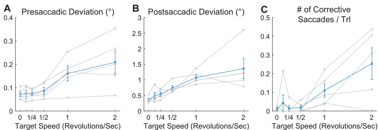
Figure 8. Measures of presaccadic and postsaccadic behavior as a function of target speed in real motion (Experiment 1). Only data from targets at 12° eccentricity are shown; thin lines indicate data from individual subjects, thick lines indicate group averages, and error bars indicate SEM. (A) Presaccadic deviation in the 100 ms prior to saccade initiation. (B) Postsaccadic deviation in the 100 ms after saccade completion. (C) Number of corrective saccades per trial in the 100 ms after saccade completion. See text for additional details.
